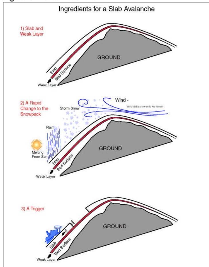
Figure 4.1-1 Slab Avalanche
