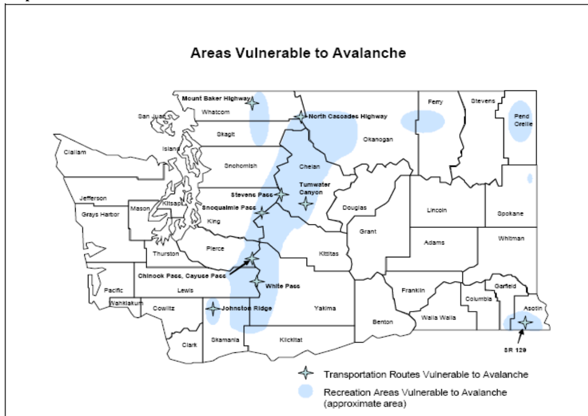
Map 4.1-1 Areas Vulnerable to Avalanche
